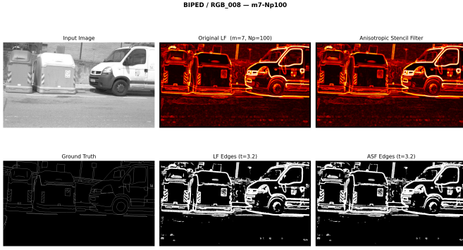
Fig. 21. Clean-data visual comparison on BIPED v1 (image 008, 1280 \times 720 ). The ASF captures fine structural details including vehicle outlines, wheel spokes, and sign text that small-kernel classical operators miss.
