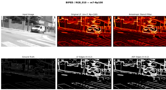
Fig. 22. Clean-data visual comparison on BIPED v1 (image 010). On this photometric-edge dataset, the ASF produces gradient maps visually competitive with deep learning outputs.
