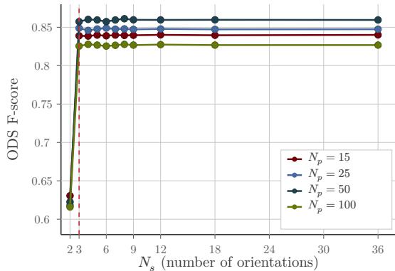
Fig. 15. ODS F-score versus number of orientations N_s at various support sizes N_p . A critical jump occurs at N_s = 3 (dashed line), where ODS increases by 0.20–0.24 relative to N_s = 2 . Beyond N_s = 3 , performance plateaus. The cliff indicates that three orientations suffice for accurate edge detection; additional orientations provide negligible benefit while multiplying computational cost.
