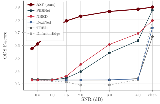
Fig. 17. ODS F-score versus signal-to-noise ratio (SNR) for the ASF and five deep learning models under Gaussian noise. The ASF (garnet) degrades gracefully as noise increases, maintaining ODS > 0.5 even at 0.3 dB SNR. Deep learning models collapse below approximately 2 dB, falling to near-random baseline (ODS \approx 0.33 ). At 1 dB SNR, the ASF achieves ODS = 0.72 while all DL models are at 0.33–0.35.
