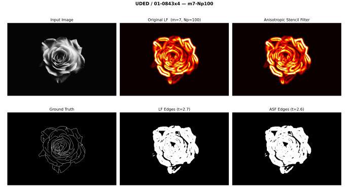
Fig. 23. Clean-data visual comparison on UDED (image 01). The ASF generalizes across diverse imaging domains without domain-specific training, detecting boundaries and internal structure.
