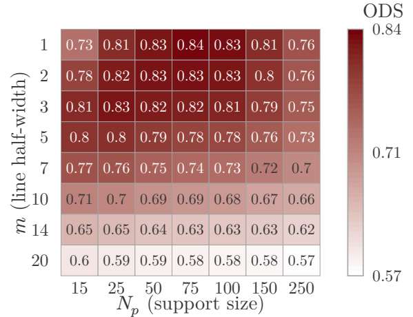
Fig. 16. LF ODS heatmap as a function of support size N_p and line half-width m . Each cell shows the ODS averaged across N_s \in \{18, 36, 72\} . The optimal region (ODS \approx 0.84 ) occurs at moderate N_p = 50 –100 and small m = 1 –3. Performance degrades with both excessive support size and excessive line extension, confirming that the published parameters ( N_p = 250 , m = 14 ) are overspecified for clean imagery.
