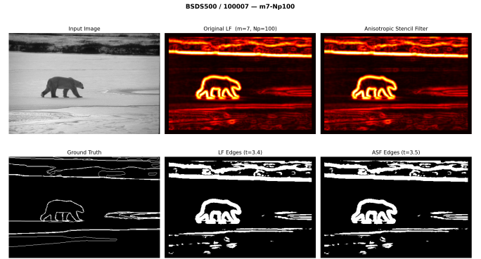
Fig. 19. Clean-data visual comparison on BSDS500 (image 100007). Top row: input image, naive LF gradient magnitude, ASF gradient magnitude (identical output, confirming mathematical equivalence). Bottom row: ground truth, LF edges, ASF edges.
