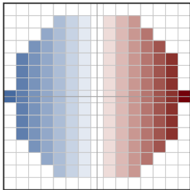
K_x^{\text{circ}}
