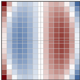
K_x^{\text{square}}
