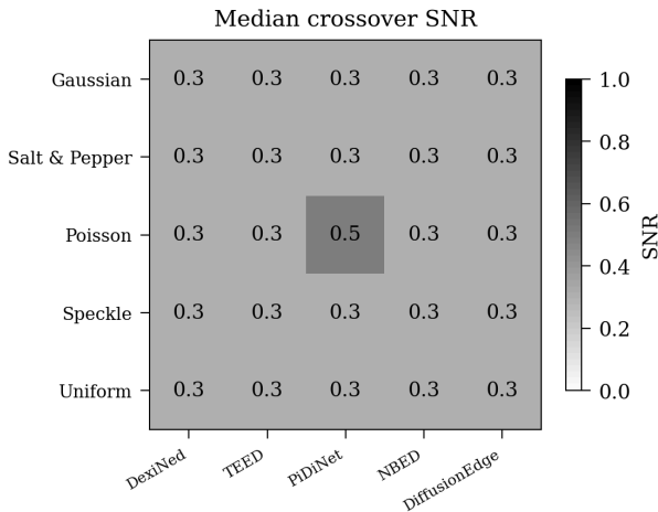
Fig. 6. Median crossover SNR by noise type and DL model. Lower values indicate earlier WVF advantage. The WVF overtakes all models at \text{SNR} \leq 0.3 –0.5, with most crossovers at \text{SNR} = 0.3 (the most extreme noise level tested).
