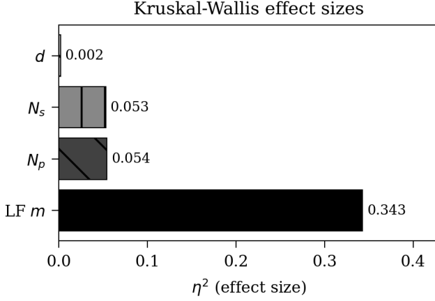
Fig. 3. Kruskal-Wallis \eta^2 effect sizes for each parameter. The LF line half-width m dominates ( \eta^2 = 0.343 ), while support size N_p and orientation count N_s have moderate effects. Polynomial order d has a negligible effect.
