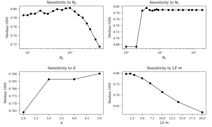
Fig. 4. Median ODS as a function of each parameter level. Top-left: N_p shows an inverted-U peaking near 80–100. Top-right: N_s saturates at 3–4. Bottom-left: d has minimal effect. Bottom-right: LF m shows monotonic decline beyond m = 2 .
