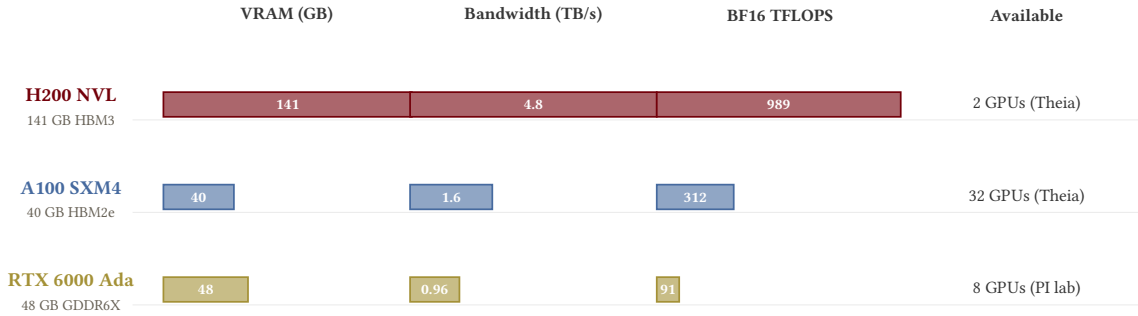
Figure 6: Comparison of available GPU resources. Memory bandwidth, not TFLOPS, is the primary determinant of RL training speed because autoregressive generation requires reading the full model weights for every token produced. The H200’s 4.8 TB/s HBM3 bandwidth makes it 3\times faster than A100 and 5\times faster than RTX 6000 Ada for generation-heavy workloads.
