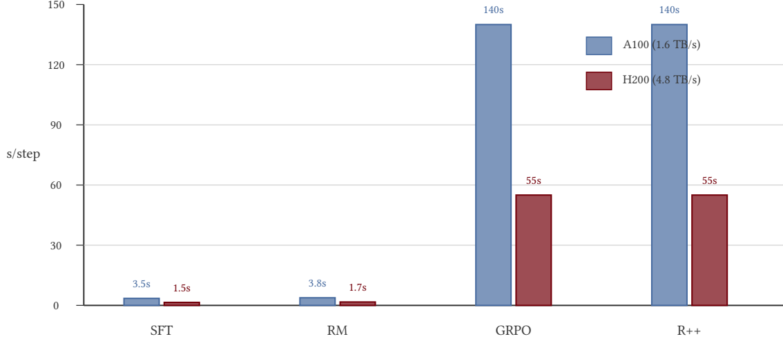
Figure 5: Per-step wall time comparison between A100 (40 GB, 1.6 TB/s) and H200 (141 GB, 4.8 TB/s). SFT and RM training are compute-bound and show minimal difference. GRPO and REINFORCE++ are generation-bound and exhibit a 2.5\times speedup on H200, directly proportional to the memory bandwidth ratio.
