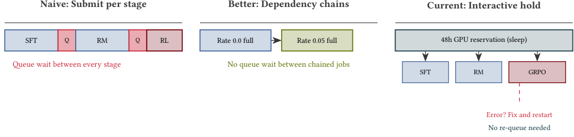
Figure 7: Evolution of SLURM scheduling strategies. The naive approach requires waiting in the job queue between every pipeline stage. Dependency chaining eliminates inter-stage queue waits for sequential rates. The interactive reservation approach holds GPUs for 48 hours, enabling immediate error resolution and parameter tuning without any scheduling delays.
