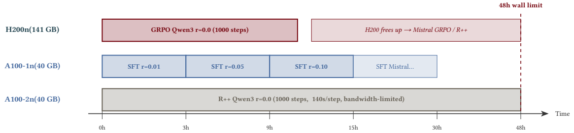
Figure 3: GPU allocation strategy for parallel training on heterogeneous hardware. The H200’s 3× higher memory bandwidth makes it essential for generation-heavy RL stages, while A100s handle compute-bound SFT training efficiently. Work is scheduled to maximize GPU utilization within SLURM’s 48-hour wall time and 5-job QOS constraints.
