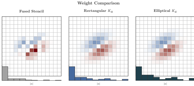
Fig. 13. Side-by-side weight comparison at \theta = 30^\circ for the three kernel variants. Left: the fused stencil weight map, showing an irregular shape with many near-zero cells. Center: the rectangular kernel, exhibiting a clean box boundary and smooth dipole weights with no near-zero interior pixels. Right: the elliptical kernel, with a smooth elliptical boundary and slightly fewer pixels. Below each weight map is a histogram of absolute weight magnitudes |\alpha| . The fused stencil histogram exhibits a pronounced spike near zero; neither geometric kernel histogram does.
