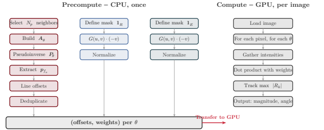
Fig. 15. Two-phase architecture overview. The precompute phase (left) runs on the CPU and differs per variant, but all three produce the same output format of (offset, weight) pairs per orientation. The compute phase (right) consumes these stencil arrays through a single variant-agnostic Triton kernel.
