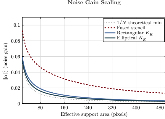
Fig. 14. Noise gain \|\alpha\|_2^2 as a function of effective support area for the three kernel variants. The theoretical minimum for a uniform kernel ( 1/N ) is shown as a dotted line. The geometric kernels track closer to the theoretical minimum across all support sizes. The fused stencil curve sits above due to its uneven weight distribution.
