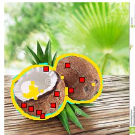
IoU = *0.96*
