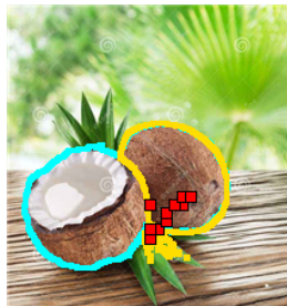
IoU = 0.41
