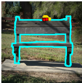
IoU = 0.00
