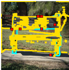
IoU = 0.16
