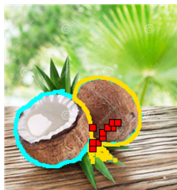
IoU = 0.41
