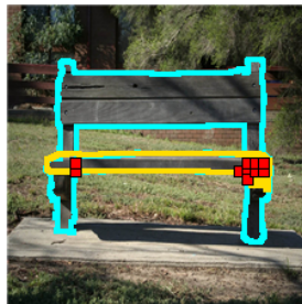
IoU = 0.21
