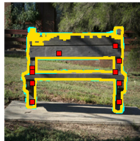
IoU = *0.92*
