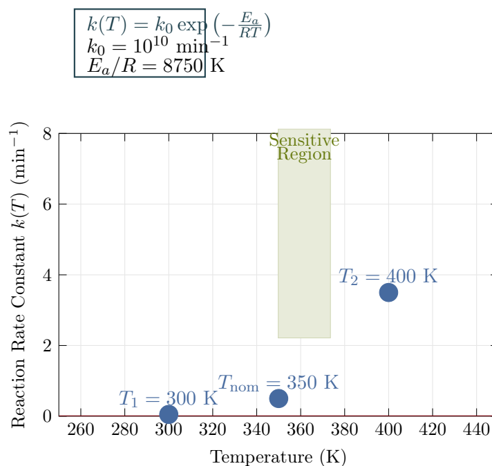
Figure 14.6: Arrhenius equation showing exponential increase in reaction rate with temperature. The nonlinear relationship creates control challenges, with the system becoming increasingly sensitive to temperature in the operating range.
