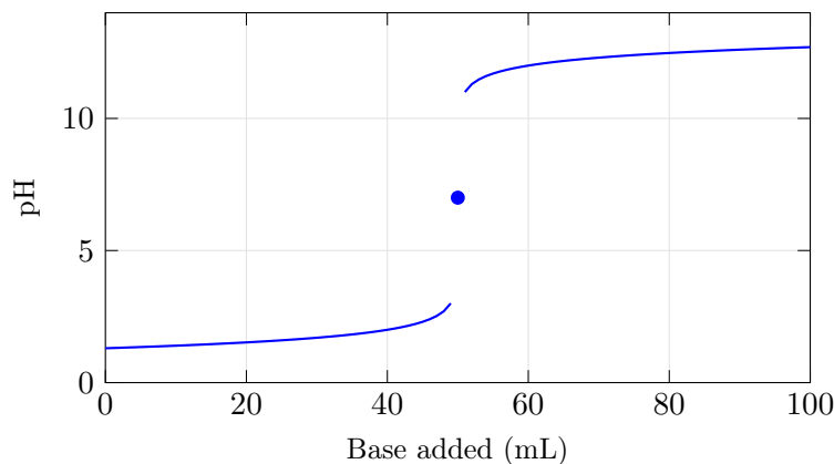
Figure 14.3: Typical pH titration curve showing high gain near equivalence.
