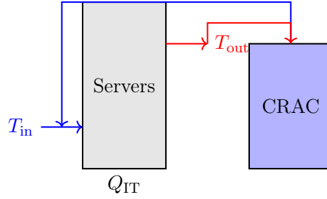
Figure 17.7: Data center thermal model.
