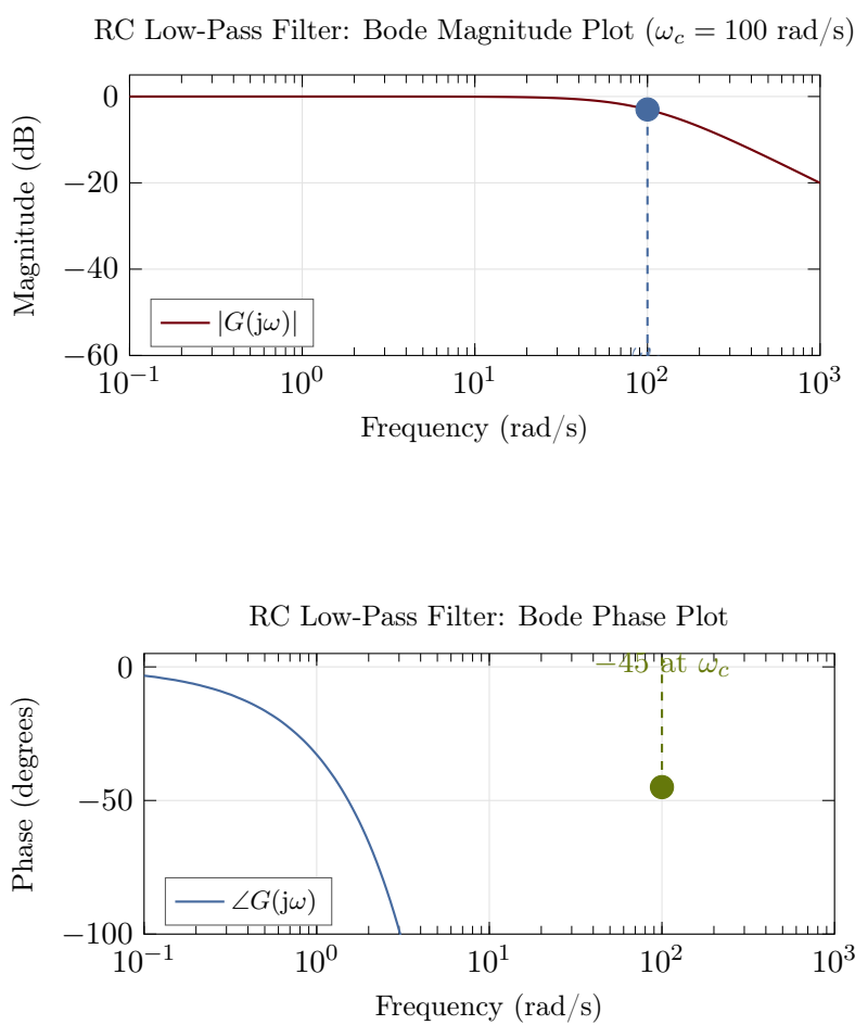
Figure 11.7: RC low-pass filter Bode plots (magnitude and phase).
