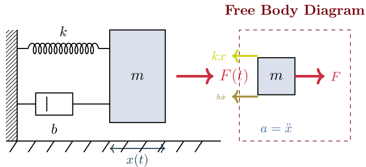
Figure 10.4: Mass-spring-damper system with free body diagram showing all forces.
