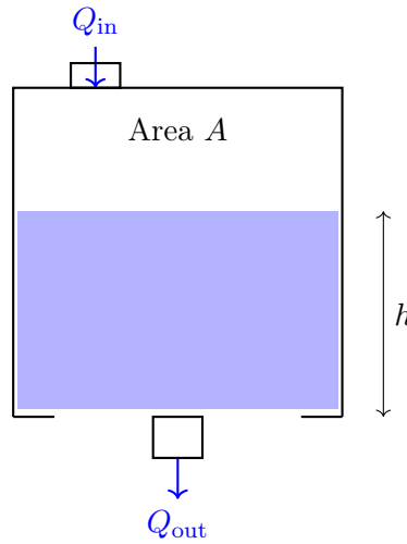
Figure 13.3: Single tank level system.
