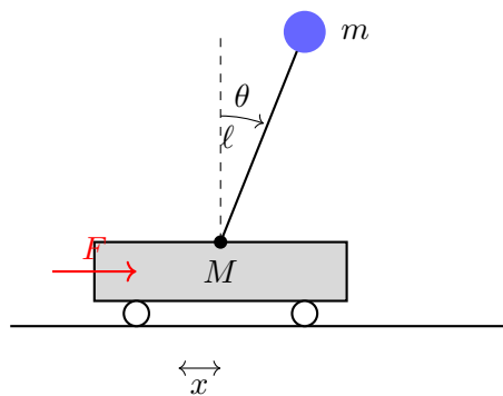
Figure 10.12: Inverted pendulum on cart.
