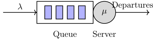
Figure 17.5: M/M/1 queue model.
