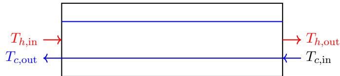
Figure 13.6: Counter-flow heat exchanger.
