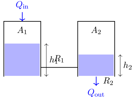
Figure 13.4: Two interacting tanks.
