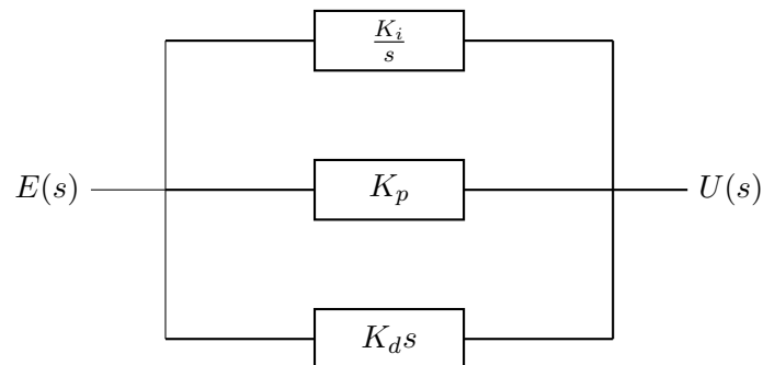
Figure 11.14: PID controller block diagram.
