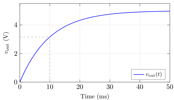
Figure 11.6: RC circuit step response.
