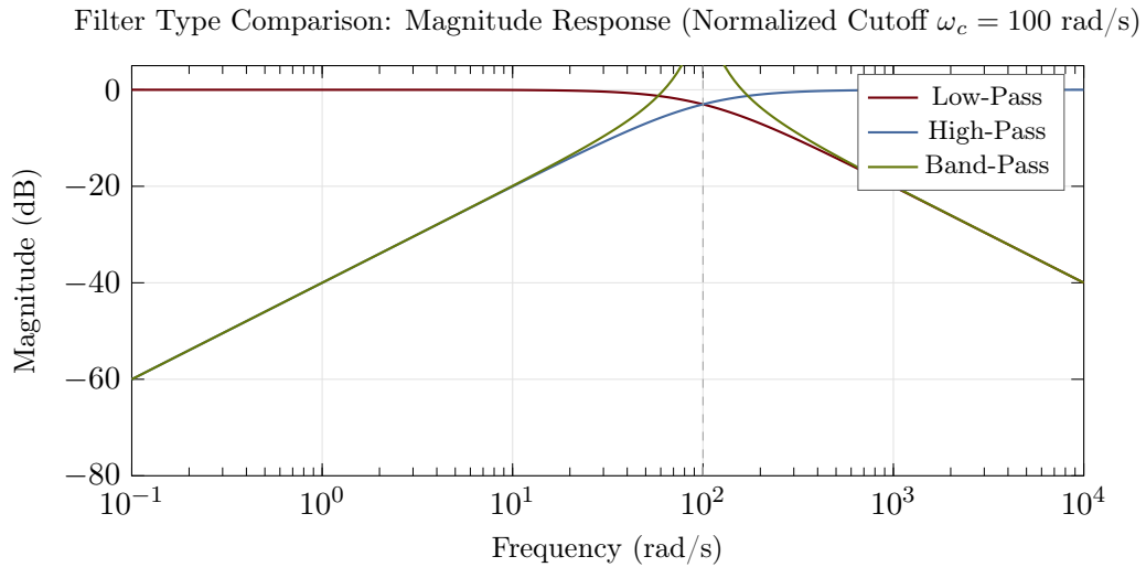
Figure 11.15: Comparison of filter types showing magnitude response of low-pass, high-pass, and band-pass filters with normalized cutoff frequency.
