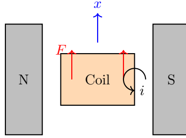
Figure 12.2: Voice coil actuator schematic.
