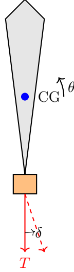
Figure 15.3: Rocket with thrust vector control.
