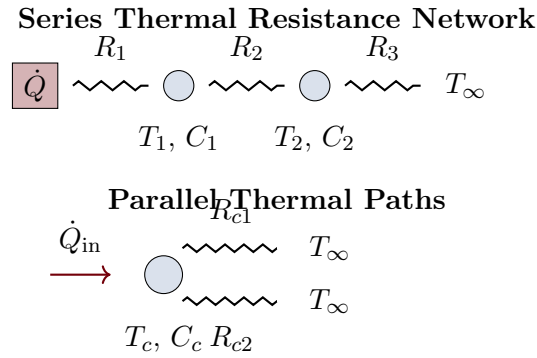
Figure 13.7: Thermal resistance networks showing series (top) and parallel (bottom) heat flow paths with thermal capacitances at nodes.
