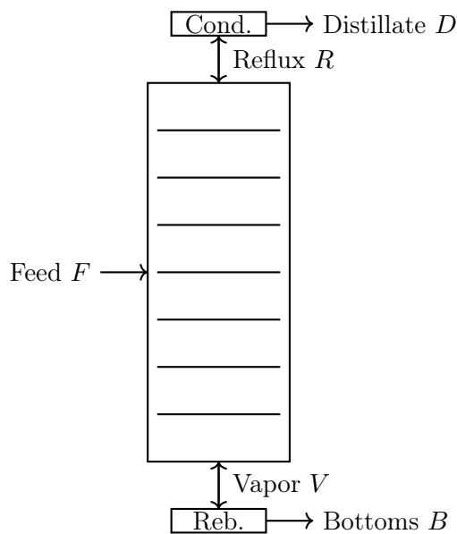
Figure 14.4: Distillation column schematic.
