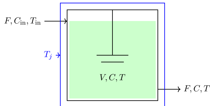
Figure 14.1: Continuous stirred-tank reactor with cooling jacket.
