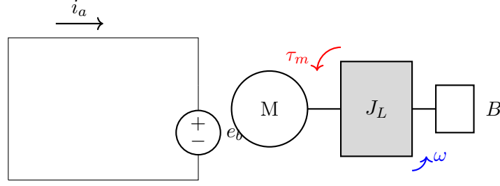
Figure 12.1: DC motor equivalent circuit and mechanical load.
