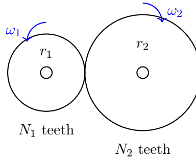
Figure 10.9: Gear pair.
