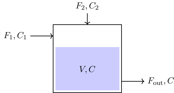
Figure 14.2: Mixing tank with two inlets.
