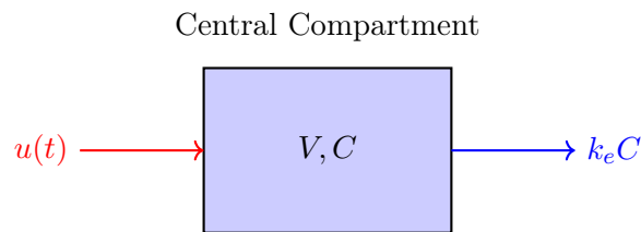
Figure 16.1: One-compartment pharmacokinetic model.
