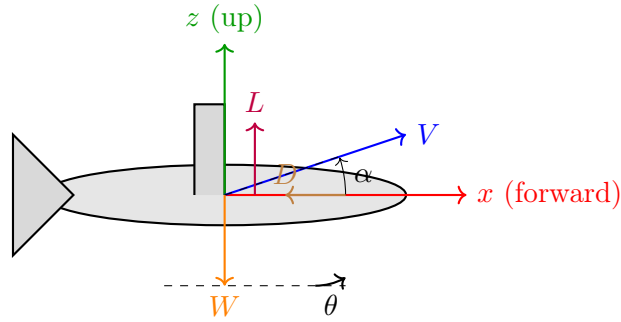
Figure 15.1: Aircraft longitudinal plane showing forces and angles.
