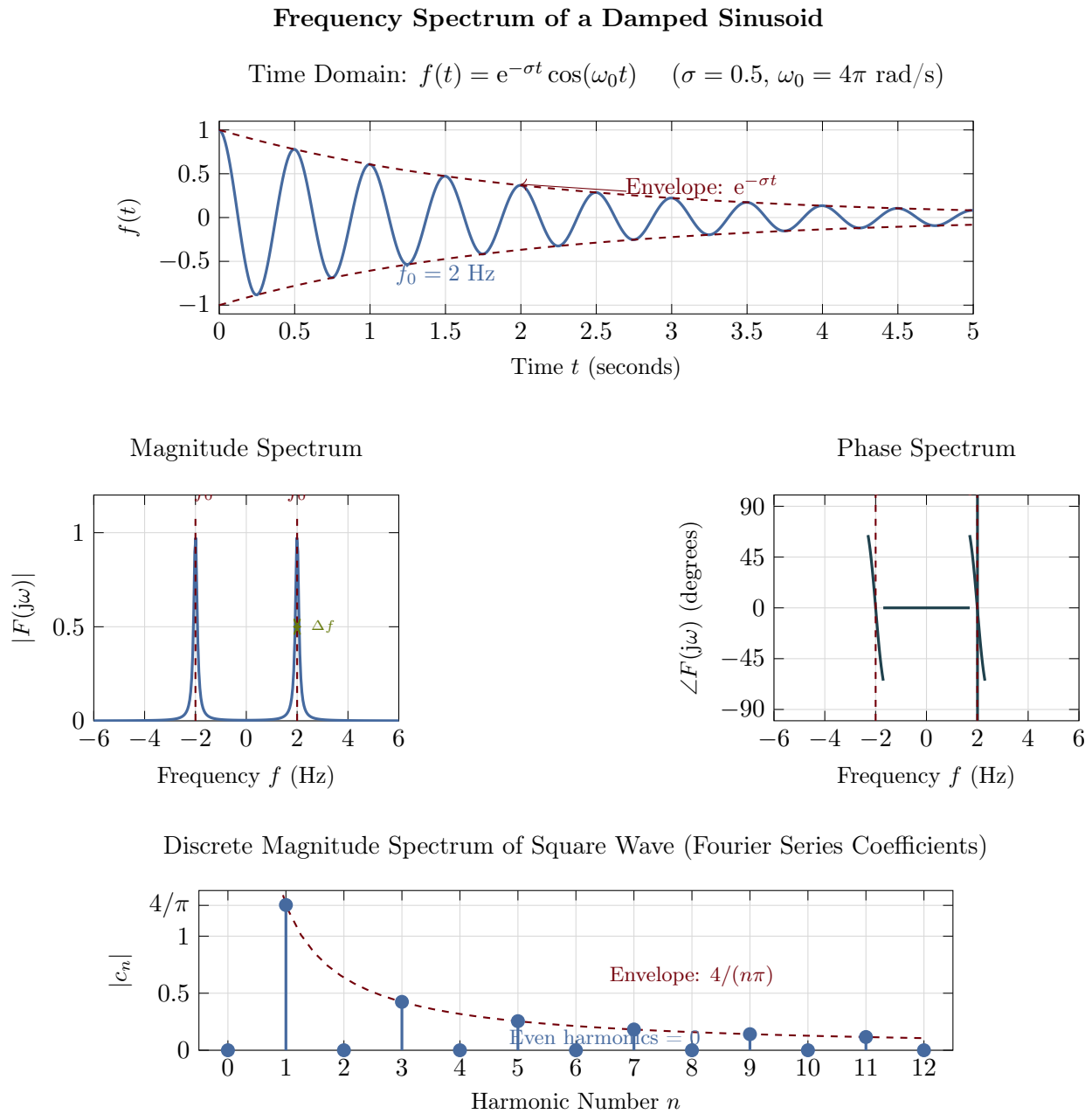
Figure 5.2: Frequency domain representation of signals. Top: Time-domain damped sinusoid f(t) = e^{-\sigma t} \cos(\omega_0 t) with decay rate \sigma = 0.5 \text{ s}^{-1} and frequency f_0 = 2 \text{ Hz} . The dashed Garnet lines show the exponential envelope. Middle: Magnitude spectrum (Atlantic blue) shows peaks at \pm f_0 with bandwidth \Delta f proportional to \sigma . Phase spectrum (Congaree teal) shows \pm 90 phase transitions at the resonance frequencies. Bottom: Discrete spectrum for a periodic square wave showing only odd harmonics with magnitude decreasing as 4/(n\pi) .
