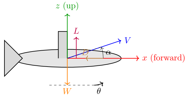
Figure 13.1: Aircraft longitudinal plane showing forces and angles.
