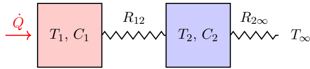
Figure 11.2: Two-capacitance thermal system.
