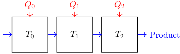
Figure 15.2: Multi-zone temperature control.
