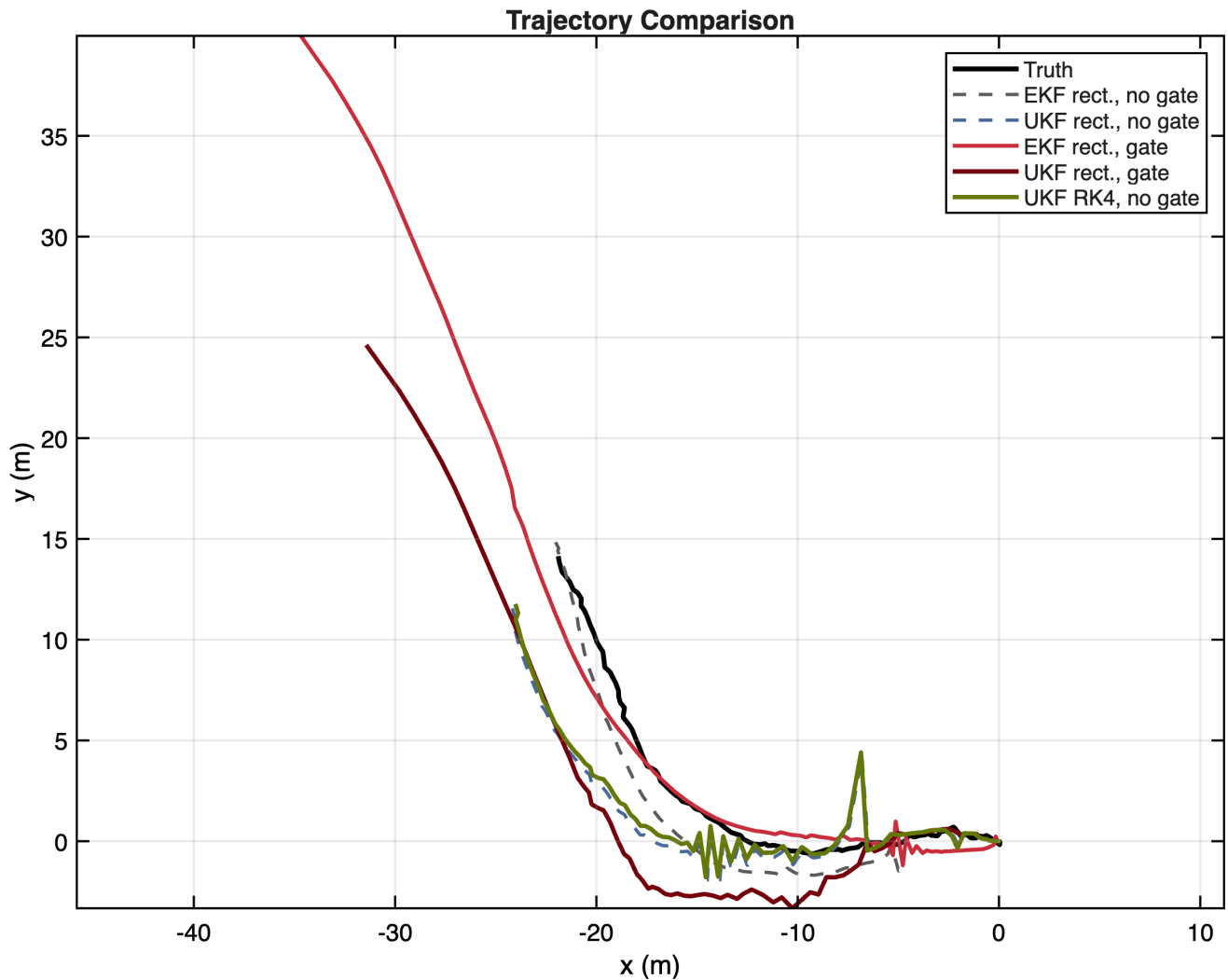
Figure 2: Trajectory comparison for the rectangular EKF and UKF baselines, the gated rectangular filters, and the ungated RK4 UKF. The ungated rectangular EKF gives the lowest position RMSE, while the gated runs drift late in the record after repeated measurement rejection.
