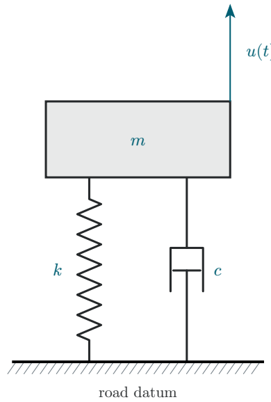
(a) Vertical spring-mass-damper idealization.
