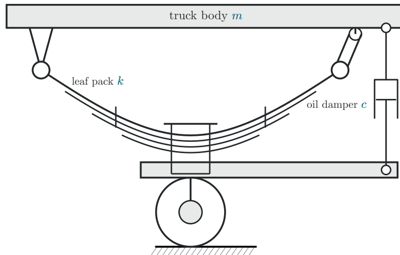
(b) Leaf-spring suspension system.
