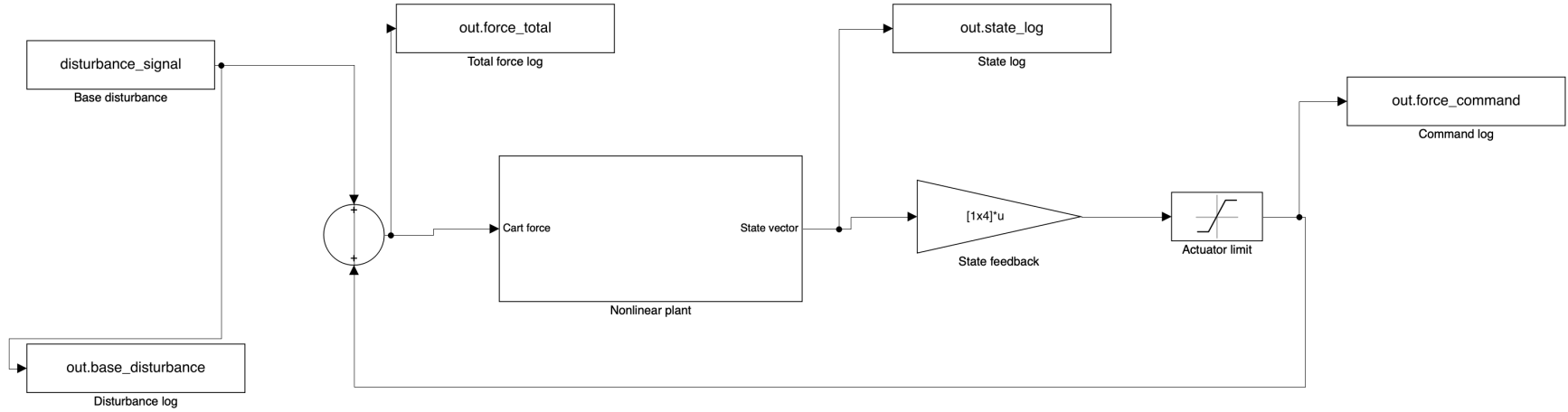
Figure 26: Complete feedback loop. The disturbance enters above the circular sum, and the limited actuator command returns below the loop.
