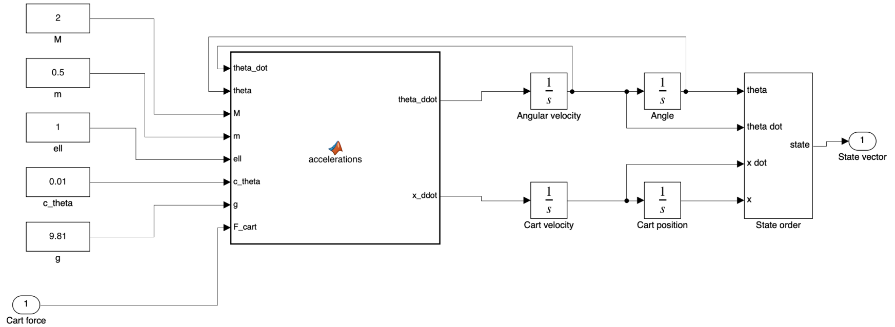
Figure 27: Nonlinear equations and four integrators retained from Project 1.
