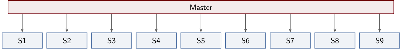
Figure 27: Flat architecture: a single master coordinates directly with every slave. The master must hold both strategic and tactical context ( \sim 80K tokens), while each slave operates with a smaller, task-specific context ( \sim 30K tokens). As the number of slaves grows, the master’s context fills with operational details, leading to context overload.
