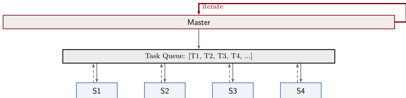
Figure 33: Master-slave pool pattern: the master enqueues tasks, slaves dequeue and execute them, and results flow back. The master can add new tasks based on results, enabling iterative batch processing.
