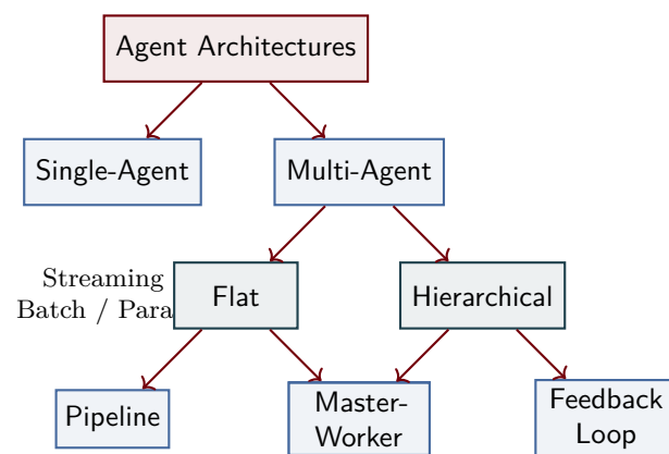
Figure 36: A taxonomy of agent architectures. Single-agent systems may operate in streaming, batch, or parallel modes but lack multi-agent coordination. Multi-agent systems divide into flat (pipeline, fan-out/fan-in) and hierarchical (master-worker, feedback loop) organizations. This taxonomy provides a structured approach to pattern selection based on control flow and task structure.
