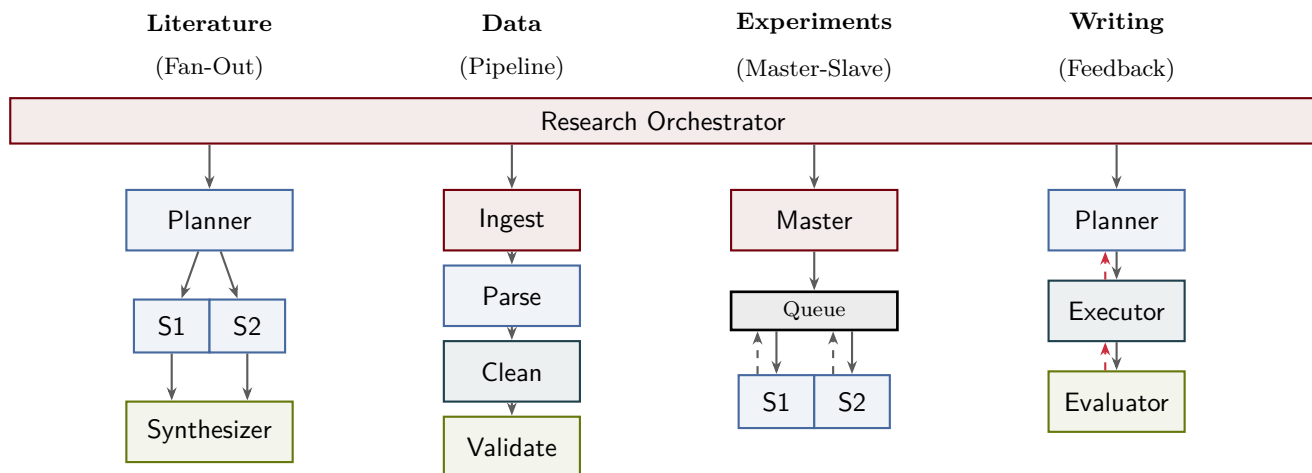
Figure 35: A composite research workflow combines four patterns under a single orchestrator. The literature phase uses fan-out to query multiple sources in parallel. The data phase pipelines ingestion, parsing, cleaning, and validation. The experiment phase employs a master-slave pool for high-throughput execution. The writing phase uses a feedback loop to iteratively refine the manuscript.
