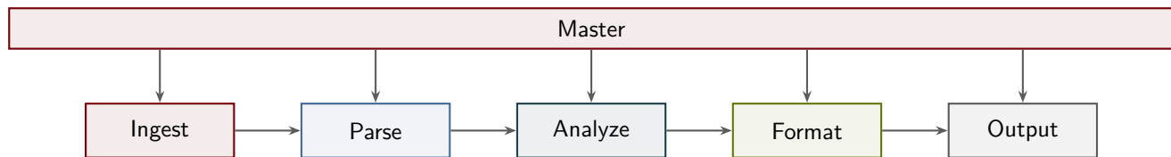
Figure 31: Pipeline pattern: data flows through a sequential chain of transformations. Each stage performs a specific operation and forwards the result to the next. The master coordinates the chain but does not participate in data transformation.
