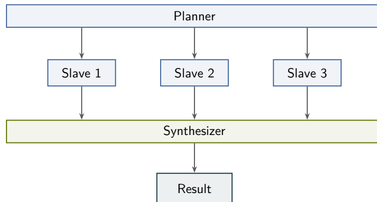
Figure 32: Fan-out/fan-in pattern: the planner decomposes work into independent subtasks and distributes them to parallel slaves. Each slave executes independently, and the synthesizer merges all results into a unified output.
