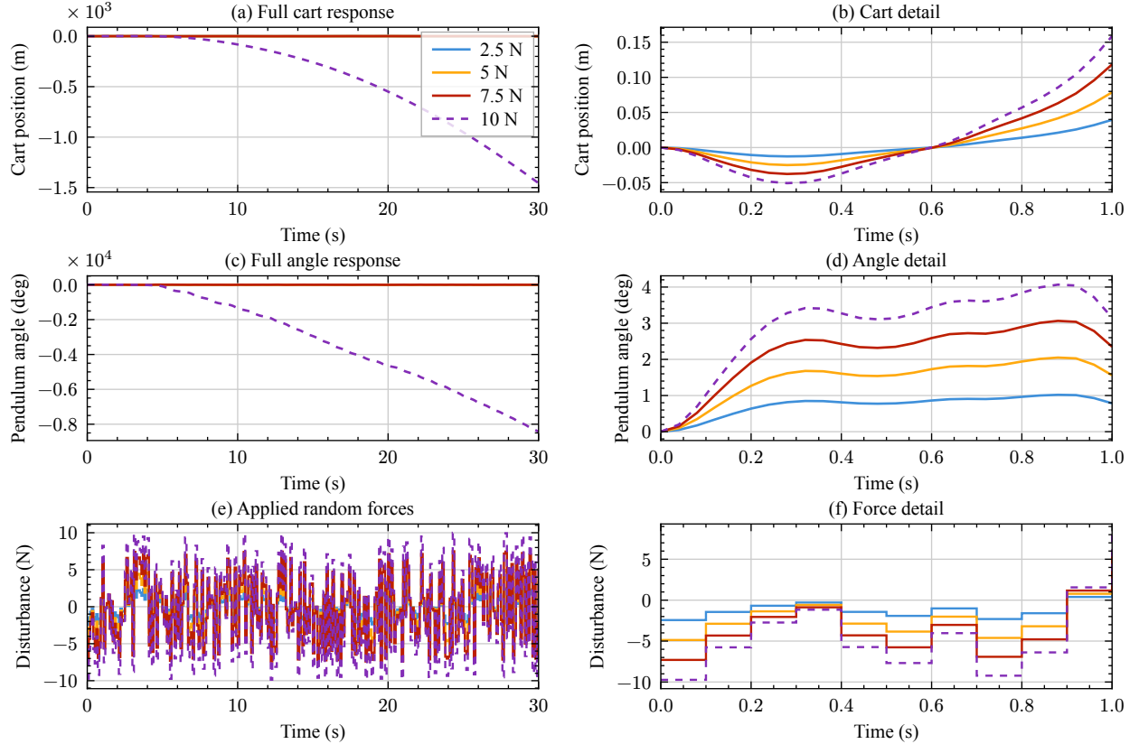
Figure 3: Random-force sweep. Every bound uses the same sequence of force draws; the 10 N case is dashed.
