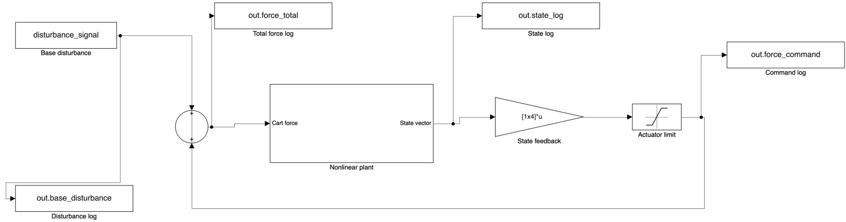
Figure 5: Complete feedback loop. The disturbance enters above the circular sum, and the limited actuator command returns below the loop.
