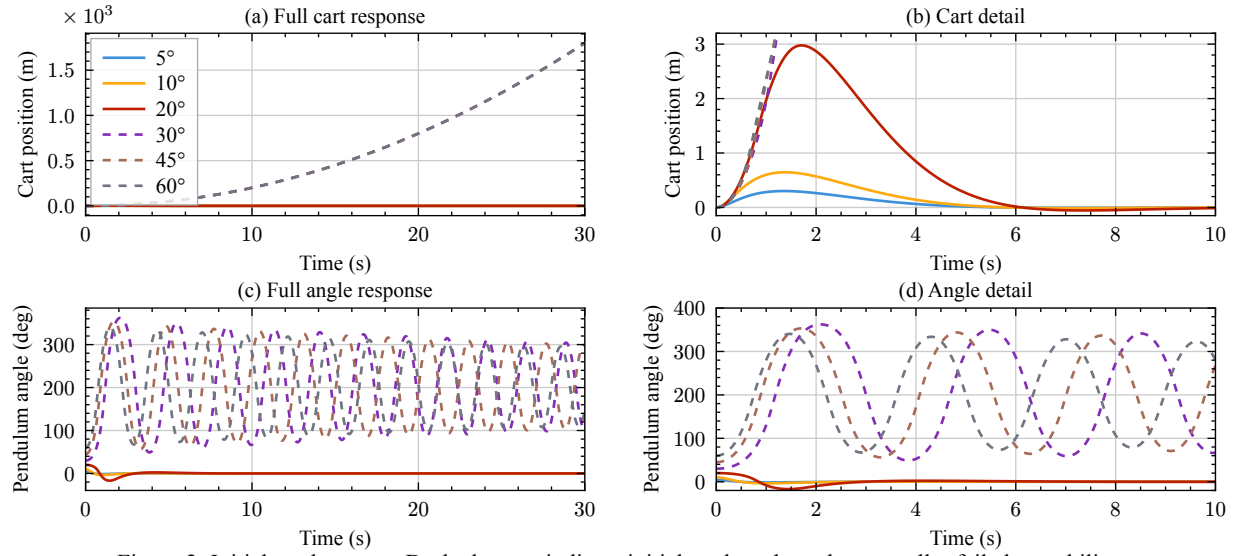
Figure 2: Initial-angle sweep. Dashed traces indicate initial angles where the controller failed to stabilize.
