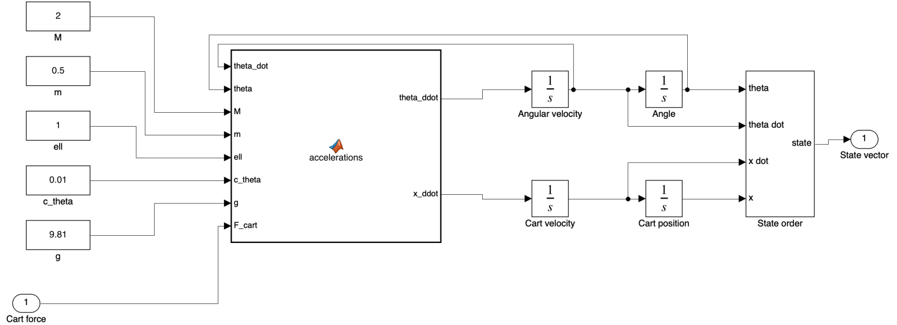
Figure 6: Nonlinear equations and four integrators retained from Project 1.
