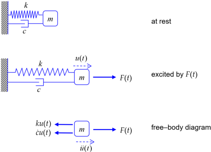
Figure 8 spring-mass-damper system excited by force F(t)
