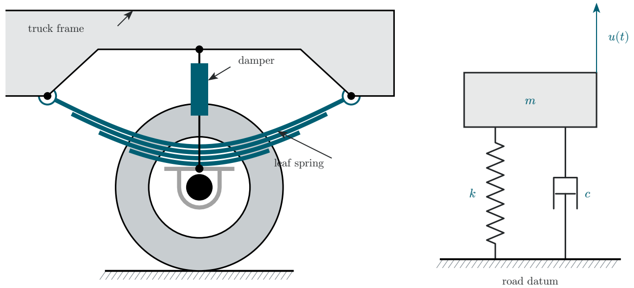
Figure 7: Truck suspension consisting of a leaf spring and an oil damper. The wheel contact is treated as the road datum in the one-degree-of-freedom idealization.
