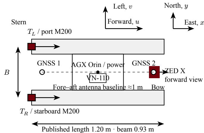
Figure 1: BlueBoat component layout in plan view. Forward is toward the bow; left is port. B is the measured separation of thrust lines, not the overall beam. Component positions are mounting proposals; heading and positive yaw are counterclockwise from east.
