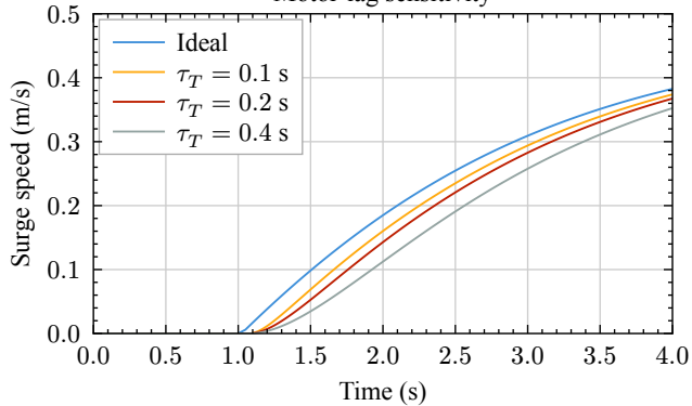
Motor-lag sensitivity
