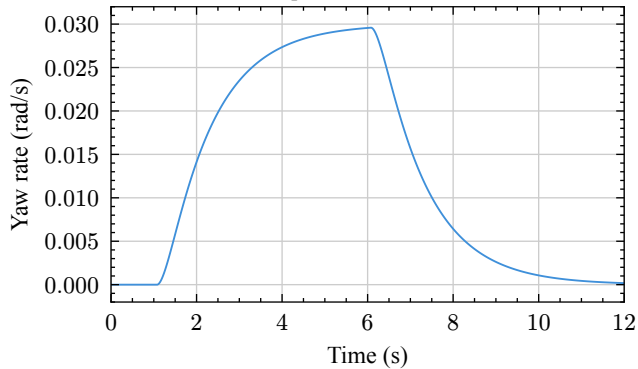
Unequal thrust then coast
