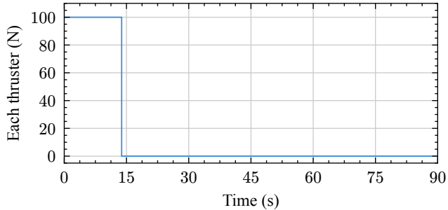
Benchmark force command
