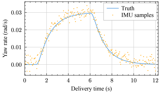
Yaw-rate measurement
