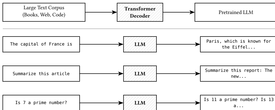
Figure 1: Stage 1: Pretraining. A transformer decoder is trained via next-token prediction on a large text corpus. The resulting model excels at text completion but cannot follow instructions or answer questions, as shown in the example inputs and outputs below the divider.
