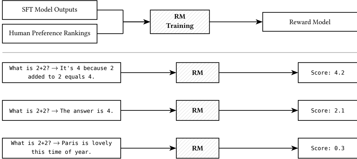
Figure 3: Stage 3: Reward Model Training. The reward model learns to score responses by quality, assigning higher values to preferred outputs.
