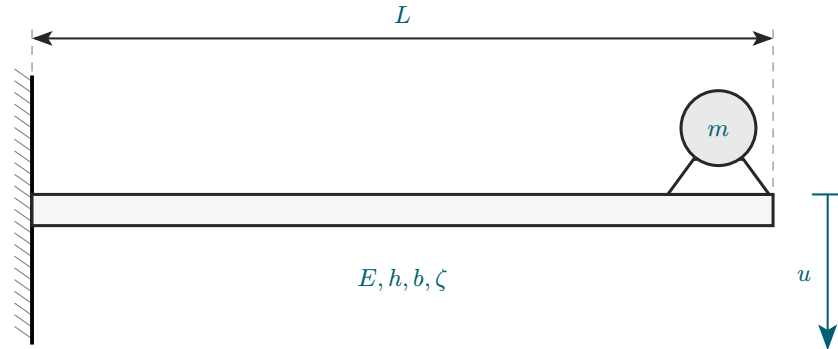
Figure 9: Damped cantilever beam excited by force F(t) from slightly unbalanced electric motor.
