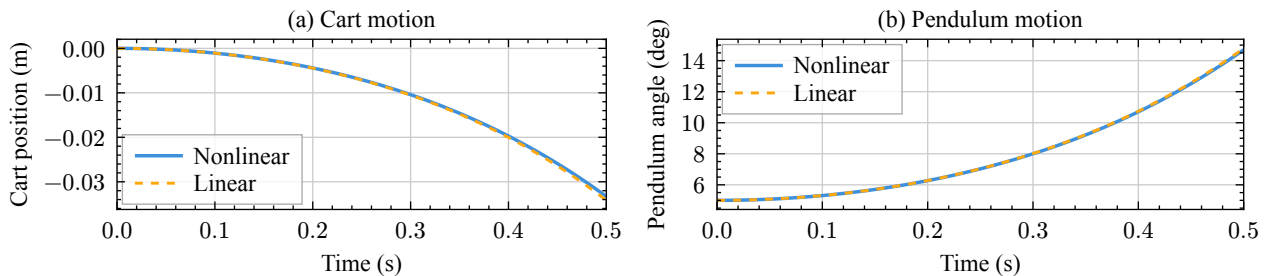
Figure 1: Linear and nonlinear responses to the same unforced 5° release over 0.5 s.
