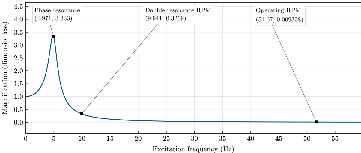
B7. Normalized frequency response, 5000 samples
