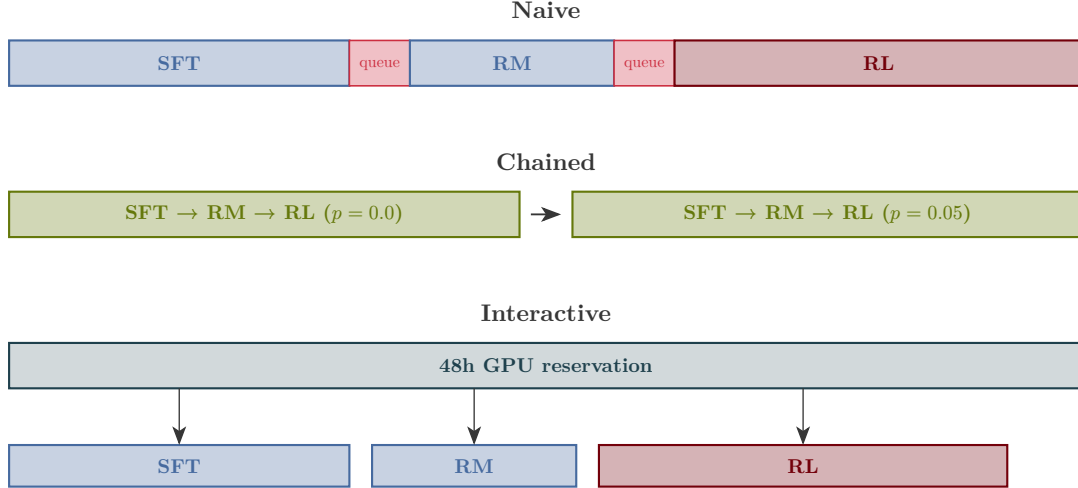
Figure 8: Evolution of SLURM scheduling strategies. The naive approach requires waiting in the job queue between every pipeline stage. Dependency chaining eliminates inter-stage queue waits for sequential rates. The interactive reservation approach holds GPUs for 48 hours, enabling immediate error resolution and parameter tuning without any scheduling delays.
