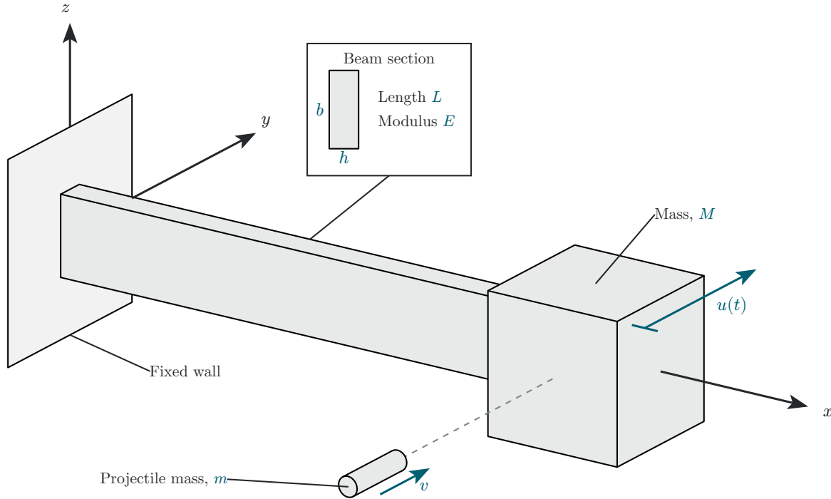
Figure 23: Impact excitation of a horizontal flex-beam vibration system.
