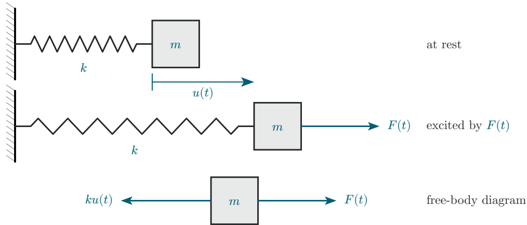
Figure 28: Spring-mass system excited by force F(t) .
