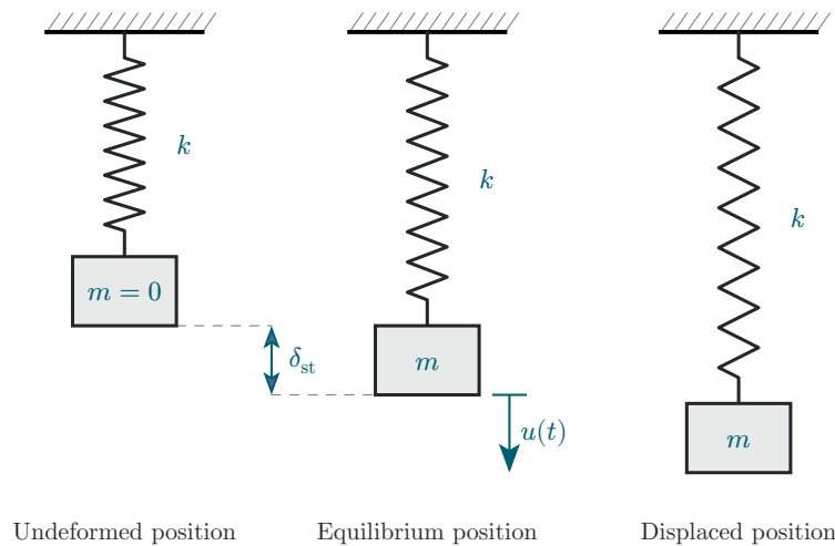
Figure 24: Vertical spring-mass vibration system.
