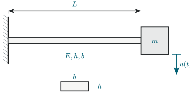
Figure 29: Cantilever beam with tip mass.
