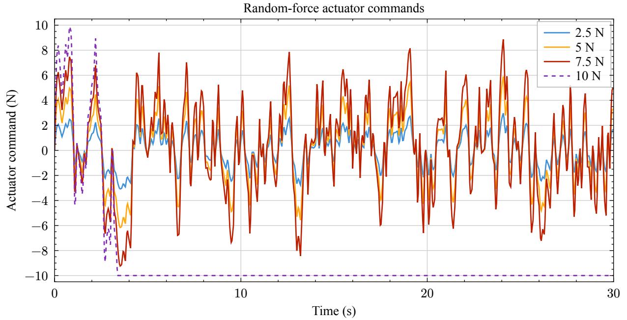
Figure 6: Actuator use under the four disturbance bounds. The dashed 10 N case loses balance and remains saturated after failure.
