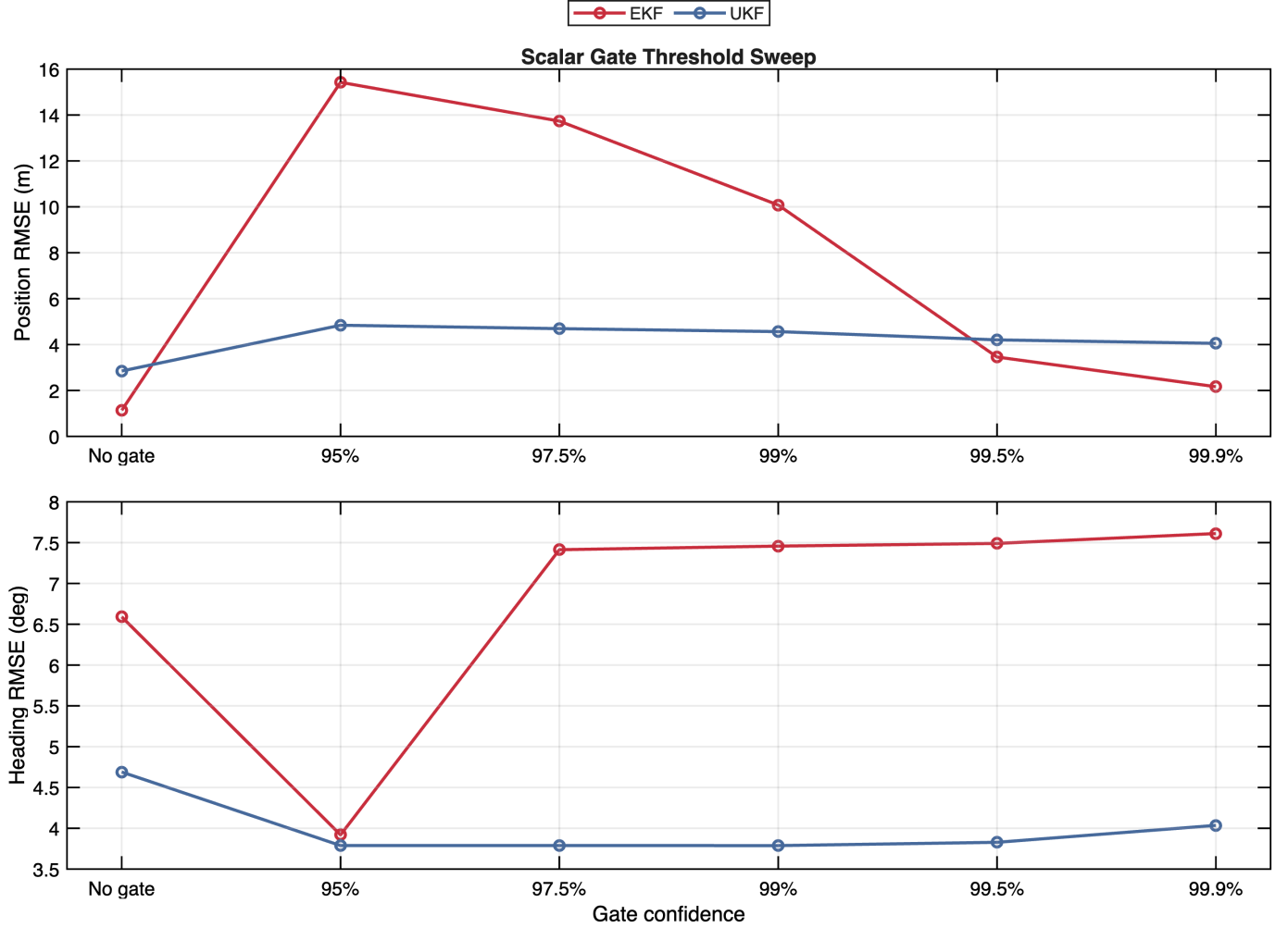
Fig. 6. Gate-threshold ablation for the rectangular EKF and UKF. Position accuracy and heading accuracy respond differently because rejecting late y_1 updates removes radial information, while rejecting isolated y_2 outliers can improve heading.
