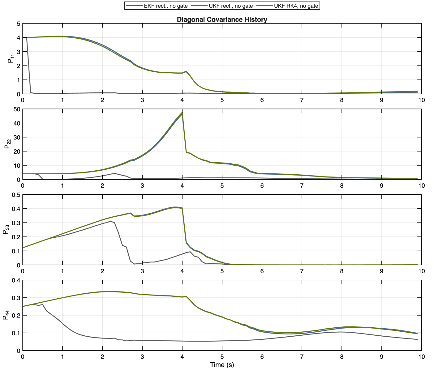
Fig. 3. Diagonal covariance histories for the rectangular EKF, rectangular UKF, and ungated RK4 UKF. The UKF variants retain visibly larger uncertainty than the EKF, while the EKF maintains the lower position RMSE in the ungated rectangular comparison.
