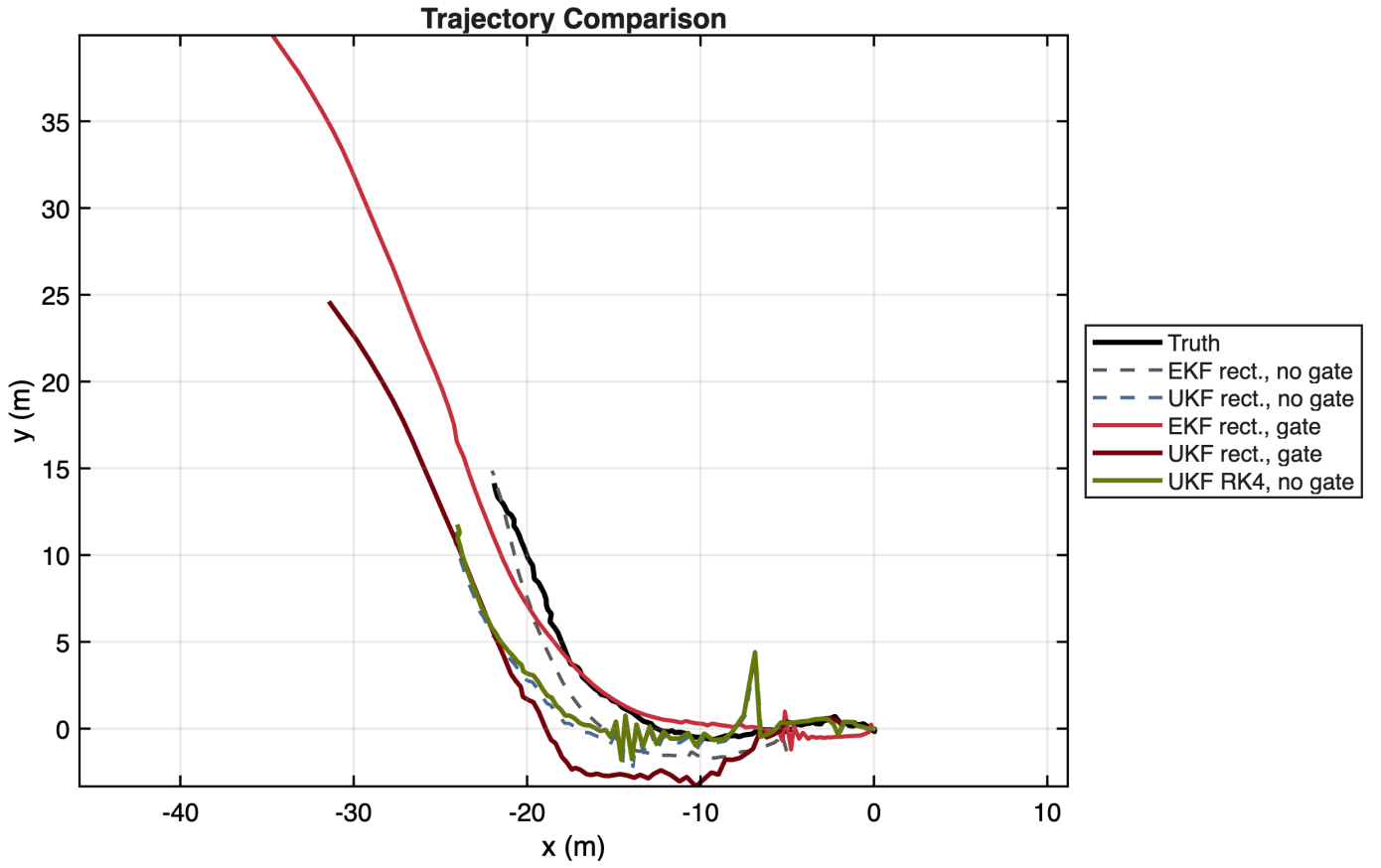
Fig. 2. Trajectory comparison for the rectangular EKF and UKF baselines, the gated rectangular filters, and the ungated RK4 UKF. The ungated rectangular EKF gives the lowest position RMSE, while the gated runs drift late in the record after repeated measurement rejection.
