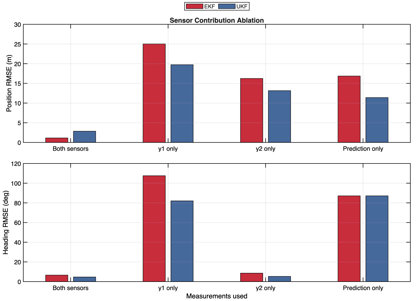
Fig. 7. Measurement-subset ablation for rectangular EKF and UKF runs. The comparison separates radial measurement information from heading measurement information and includes a prediction-only baseline.
