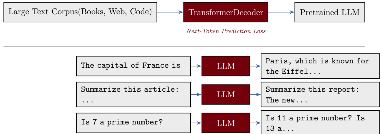
Figure 1: Stage 1: Pretraining. A transformer decoder is trained via next-token prediction on a large text corpus. The resulting model excels at text completion but cannot follow instructions or answer questions, as shown in the example inputs and outputs below the divider.
