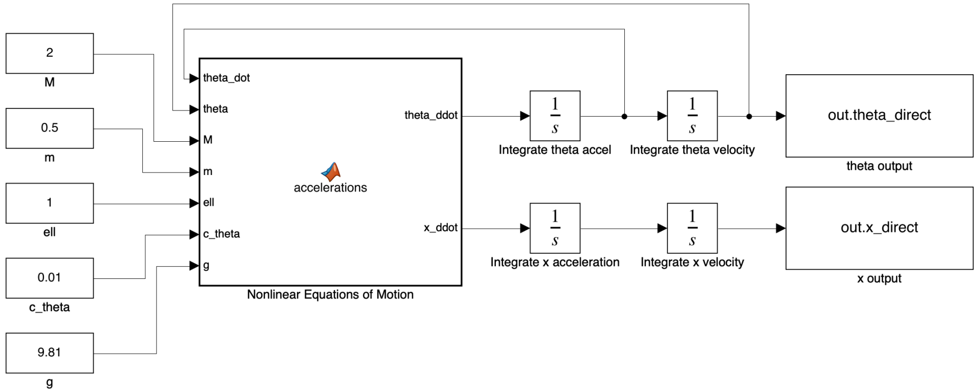
Figure 2: Editable Simulink implementation of the nonlinear mass-matrix equations.
