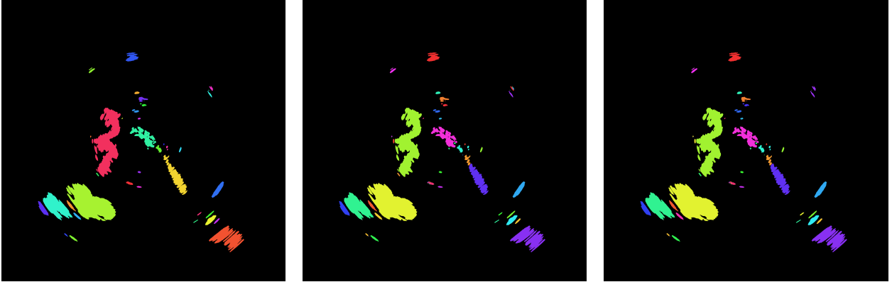
Fig. 4 Clustering results comparison on synthetic radar data (frame 25 of 50). Each color represents a distinct cluster. Left: Vanilla DBSCAN ( \varepsilon_s = 10 ) produces 1693 clusters with many small spurious detections from noise. Center: Adaptive ST-DBSCAN ( \varepsilon_{\min} = 20 ) produces 1177 clusters through larger spatial neighborhoods. Right: Adaptive + Gap Recovery merges temporally adjacent clusters, consolidating fragments into more continuous regions.
