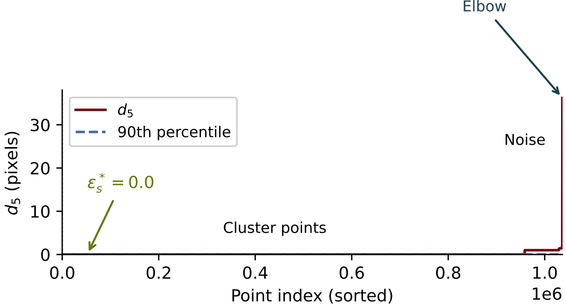
Fig. 2 Sorted k-nearest-neighbor distances for a representative radar frame ( k = 5 ). The elbow in the curve indicates the transition between dense cluster regions (low k-distance) and sparse noise regions (high k-distance). The 90th percentile threshold (dashed line) provides an adaptive epsilon that separates cluster points from noise.
