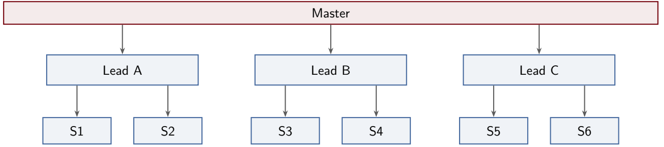
Figure 28: Layered architecture: the master ( \sim 15\text{K} tokens) delegates to intermediate leads ( \sim 50\text{K} tokens each), who each manage a subset of slaves ( \sim 30\text{K} tokens each). Each lead acts as both a slave (to the master above) and a master (to its slaves below). No single agent must hold the entire system state.
