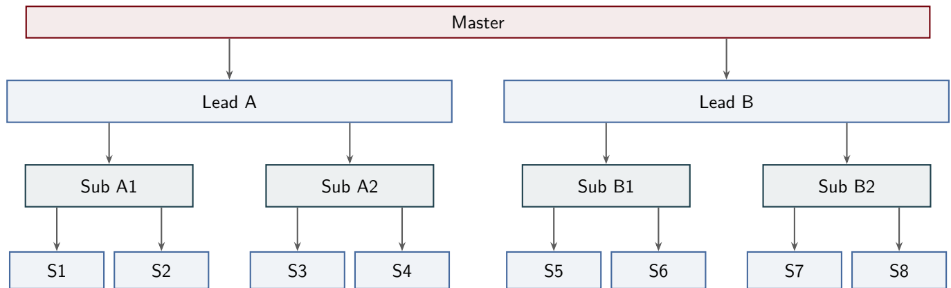
Figure 29: Deep architecture: four layers with hierarchical branching. Master delegates to 2 leads, each lead manages 2 sub-leads, and each sub-lead coordinates 2 slaves. Three sequential handoffs are required to reach execution. Best for complex decomposition requiring hierarchical refinement.
