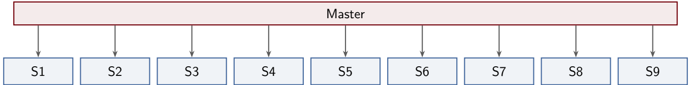
Figure 27: Flat architecture: a single master coordinates directly with every slave. The master must hold both strategic and tactical context ( \sim 80\text{K} tokens), while each slave operates with a smaller, task-specific context ( \sim 30\text{K} tokens). As the number of slaves grows, the master’s context fills with operational details, leading to context overload.
