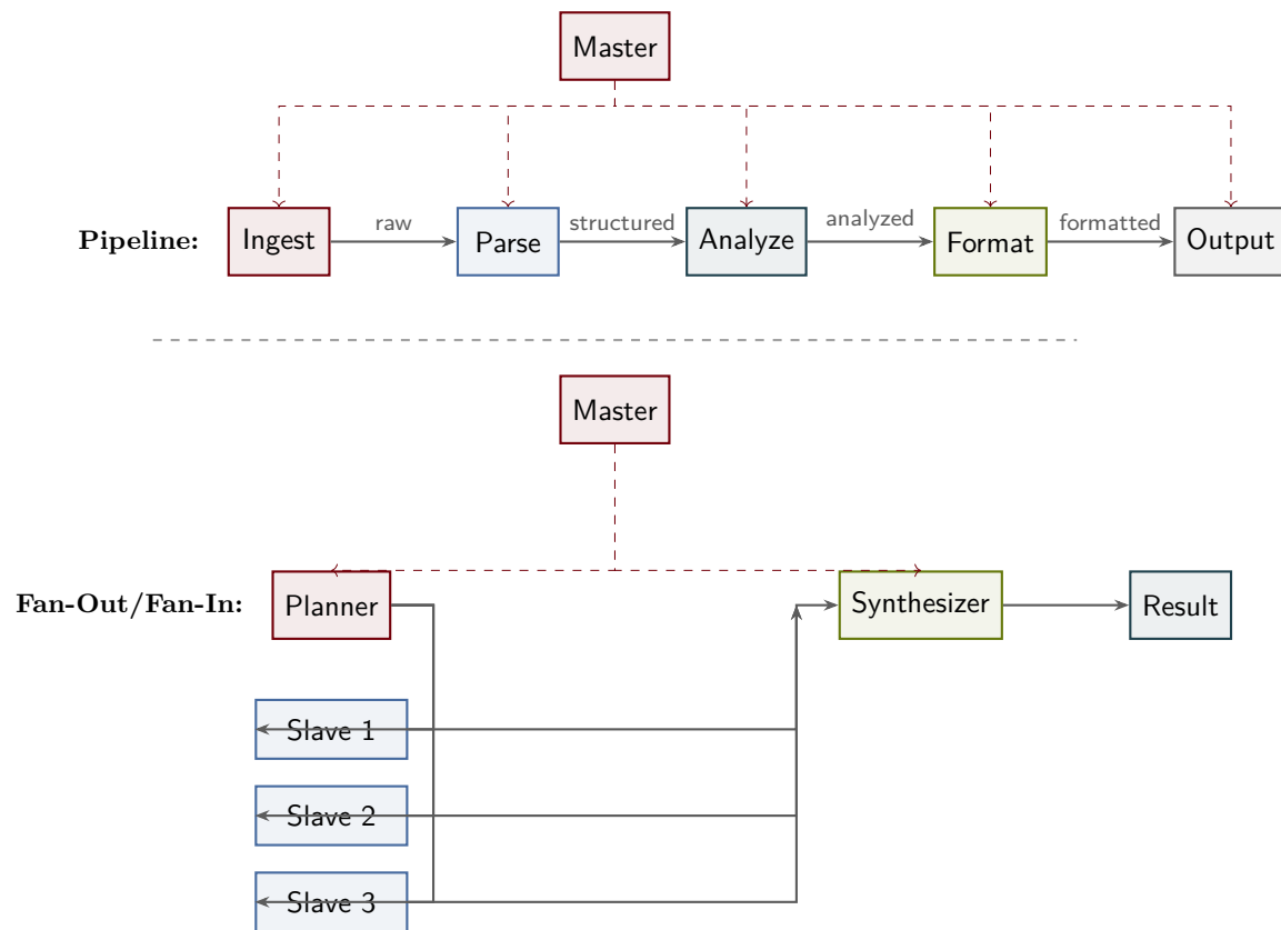
Figure 31: Top: The pipeline pattern processes data through a sequential chain of transformations. Each stage performs a specific operation and forwards the result to the next stage. The master coordinates the chain but does not participate in data transformation. Bottom: The fan-out/fan-in pattern distributes independent subtasks to parallel slaves. The planner decomposes the problem, slaves execute in parallel, and the synthesizer merges results.
