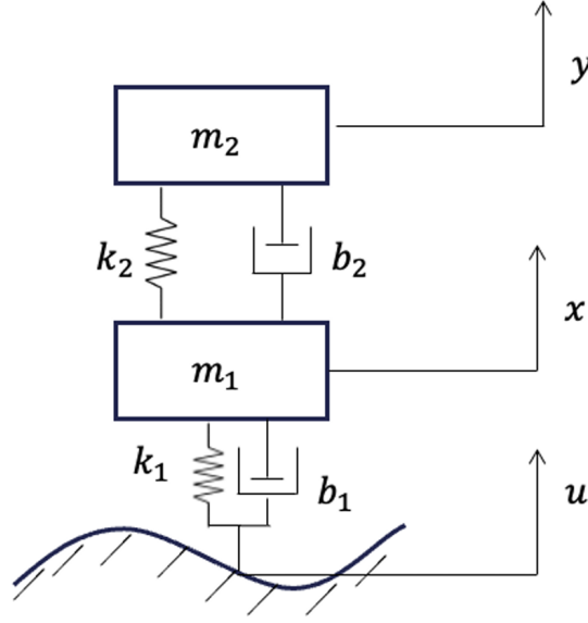
Figure 6: Suspension System
