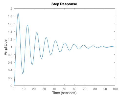
Figure 8: Step Response over 100 Seconds
