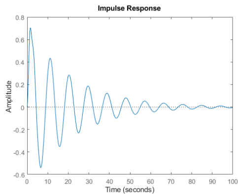
Figure 7: Impulse Response over 100 Seconds
