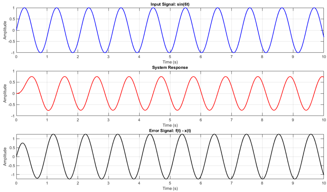
Figure 9: Time response of the system and the error signal for the input \sin(6t) .
