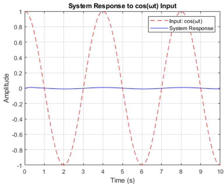
Figure 3: System Response to Cosine Input
