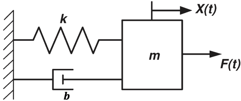
Figure 1: Spring-Mass-Damper System
