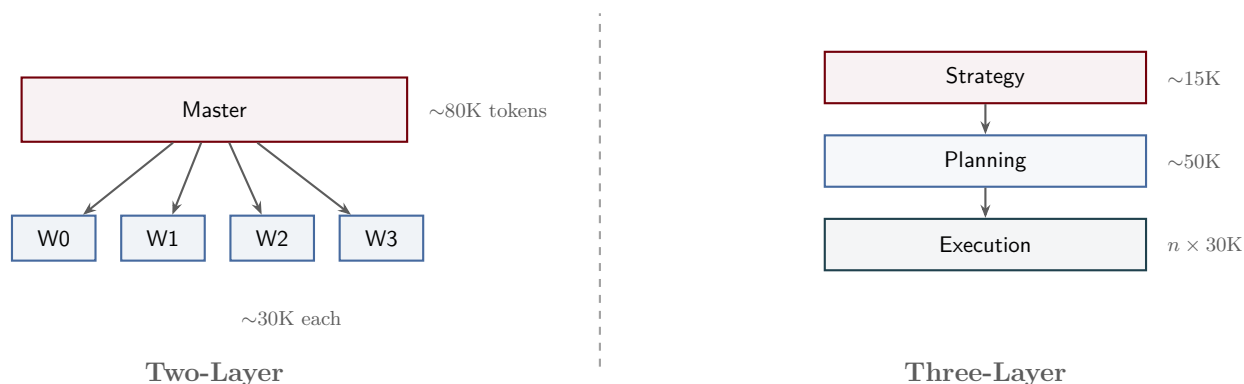
Figure 25: Comparison of two-layer and three-layer agent architectures. The two-layer system places all strategic and tactical reasoning in a single master, consuming a large context budget. The three-layer system separates strategy from planning, allowing each layer to operate within a smaller, more focused context window. The execution layer scales horizontally by adding slaves as needed.
