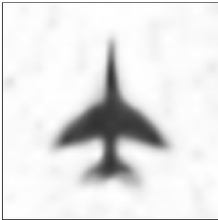
Super-Resolution (EDSR)
