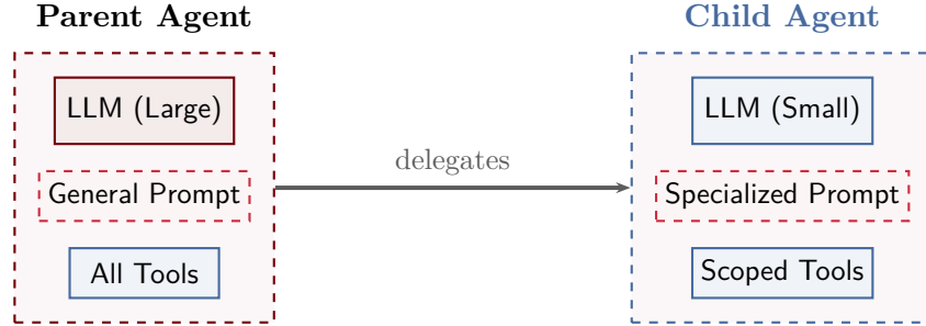
Figure 8: A sub-agent shares the same architecture as a standard agent (Section 3) but differs in its model selection, system prompt specialization, and tool access scope.
