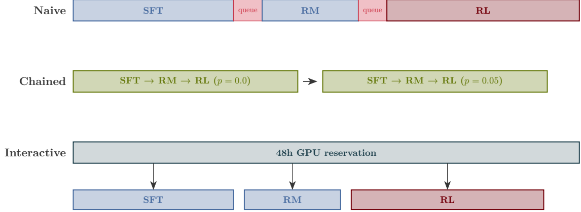
Figure 9: Evolution of SLURM scheduling strategies. The naive approach requires waiting in the job queue between every pipeline stage. Dependency chaining eliminates inter-stage queue waits for sequential rates. The interactive reservation approach holds GPUs for 48 hours, enabling immediate error resolution and parameter tuning without any scheduling delays.
