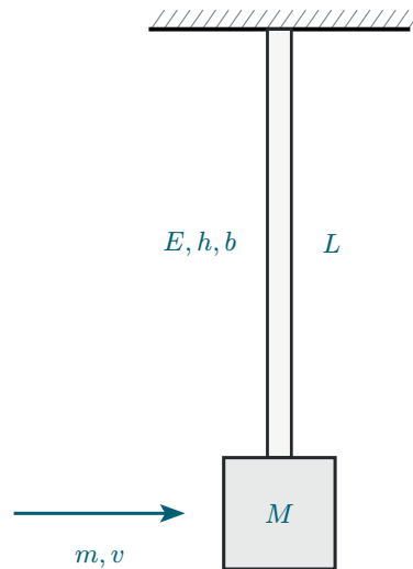
Figure 42: Impact excitation of a vertical flex-beam pendulum.
