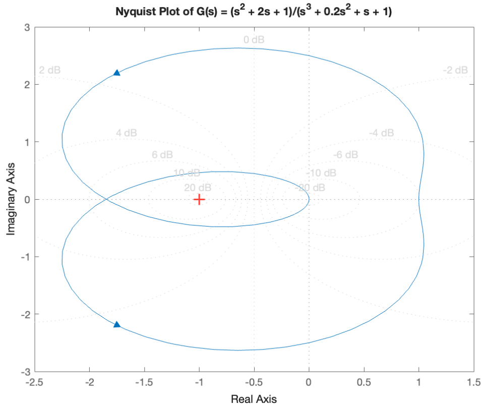
Figure 5: Nyquist Plot from MATLAB
