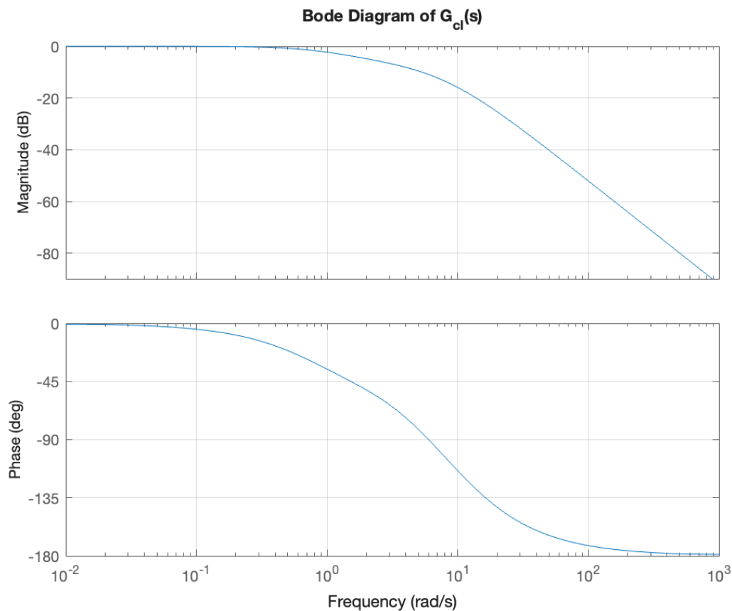
Figure 3: Bode Magnitude Plot from MATLAB
