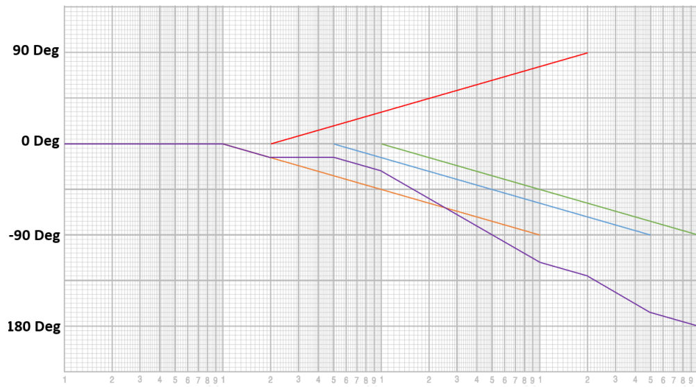
Figure 2: Bode Phase Plot
