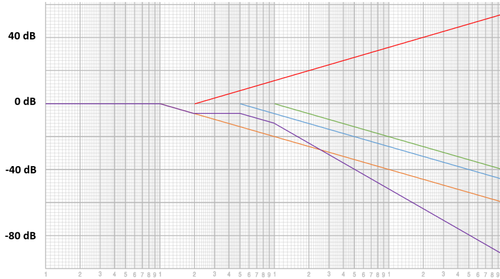
Figure 1: Bode Magnitude Plot
