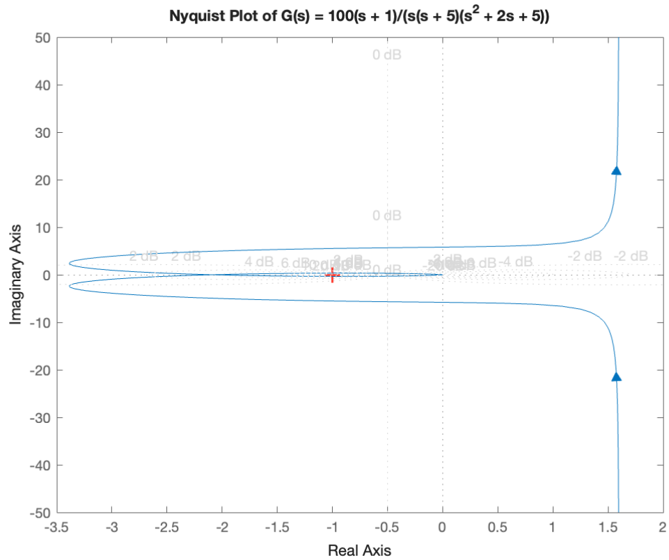
Figure 6: Nyquist Plot from MATLAB
