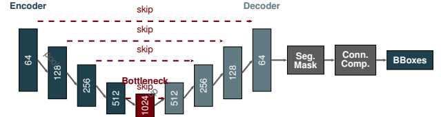
Fig. 10. U-Net encoder-decoder architecture with skip connections for per-pixel radar target segmentation.
