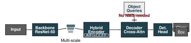
Fig. 11. RT-DETR transformer-based detector. End-to-end detection without NMS post-processing via learned object queries and cross-attention decoding.
