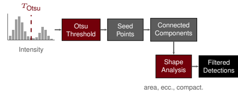
Fig. 7. Otsu thresholding with region property analysis. Seed-point detection handles the small-target problem before shape-based filtering.
