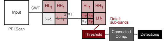
Fig. 6. Two-level 2D wavelet decomposition (DWT layout shown for clarity; SWT preserves full spatial resolution). Target energy concentrates in detail sub-bands (garnet), which are thresholded to produce detections.
