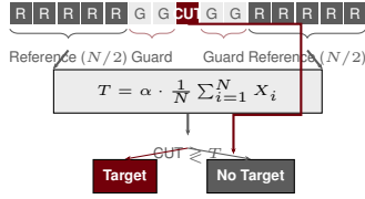
Fig. 4. CA-CFAR detector sliding window architecture (1D cross-section). The cell under test (CUT) is compared against an adaptive threshold derived from surrounding reference cells.
