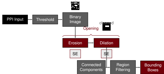
Fig. 5. Morphological detection pipeline. Structuring element operations remove noise before connected component extraction.
