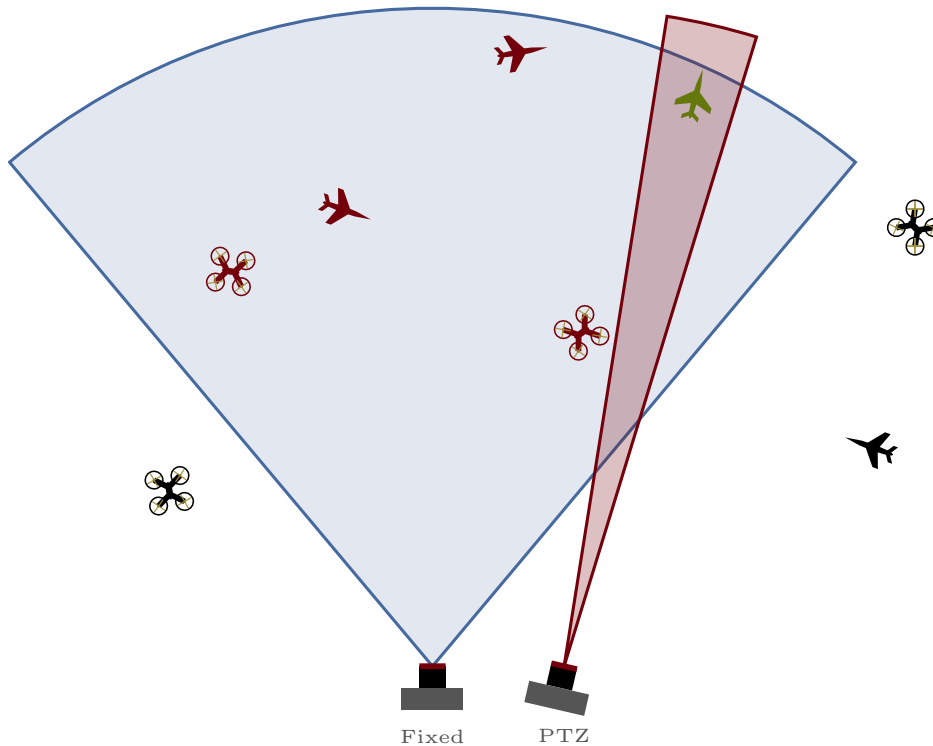
Fig. 4 Field of view comparison. The wide camera (blue) covers approximately 90^\circ for persistent surveillance, while the PTZ camera (red) provides a narrow, steerable view.
