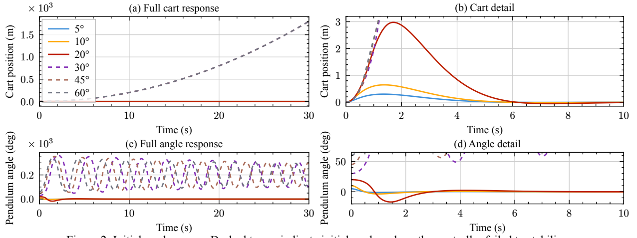
Figure 2: Initial-angle sweep. Dashed traces indicate initial angles where the controller failed to stabilize.
