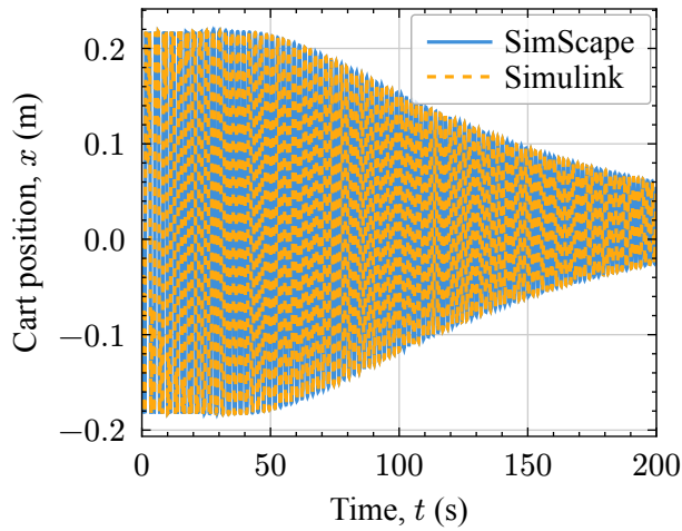
Figure 3: Cart position over 200 s.
