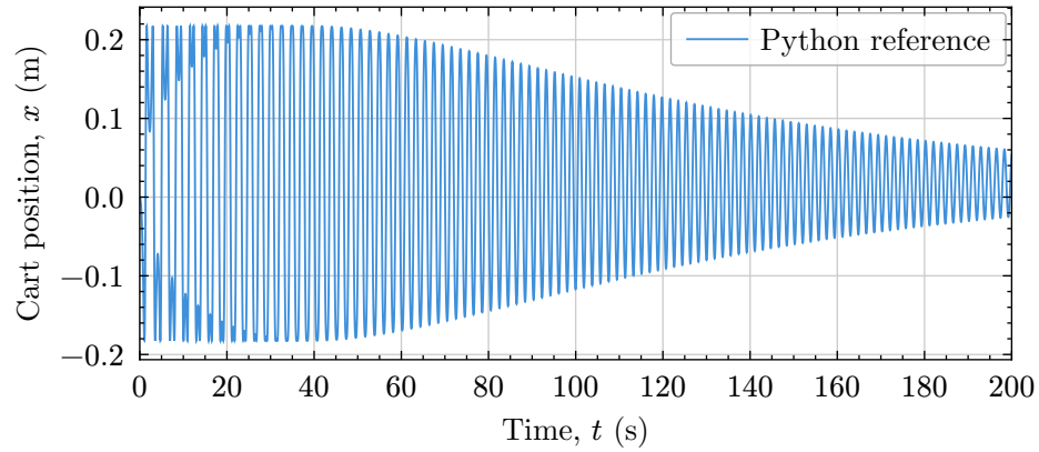
Figure 3: Cart position over 200 s.
