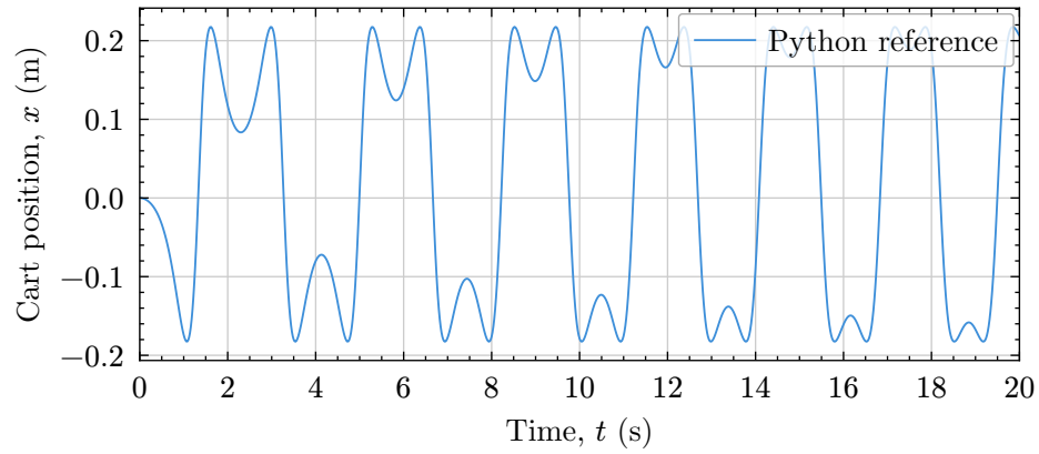
Figure 1: Cart position over 20 s.
