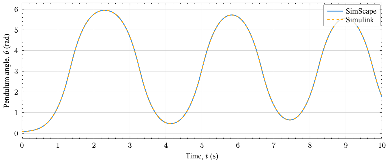
Figure 2: Pendulum angle over 10 s.
