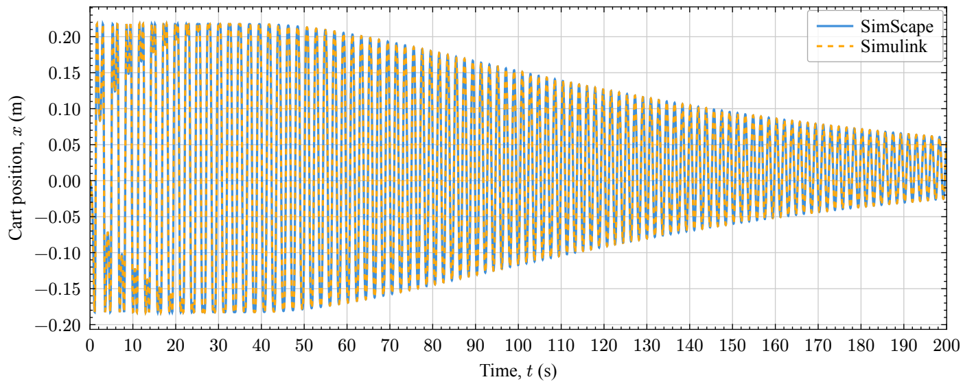
Figure 3: Cart position over 200 s.
