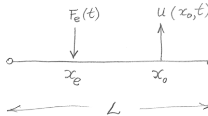
Figure 4 Struck string: (a) the hammered dulcimer; (b) schematic
