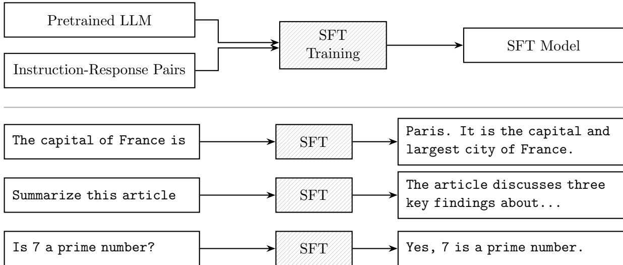
Figure 2: Stage 2: Supervised Fine-Tuning. The resulting SFT model can follow instructions, summarize text, and answer questions directly.
