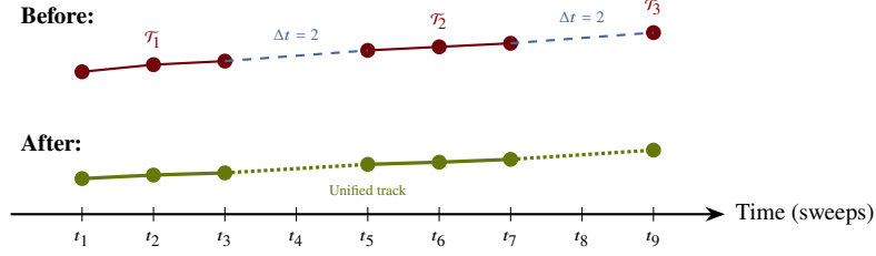
Fig. 3 Gap recovery mechanism. Before recovery (top): intermittent target returns create three disjoint cluster fragments \mathcal{T}_1, \mathcal{T}_2, \mathcal{T}_3 . After recovery (bottom): fragments within the temporal threshold \tau and spatial threshold d_{\max} are merged via Union-Find, restoring track continuity (dotted lines indicate interpolated gaps).
